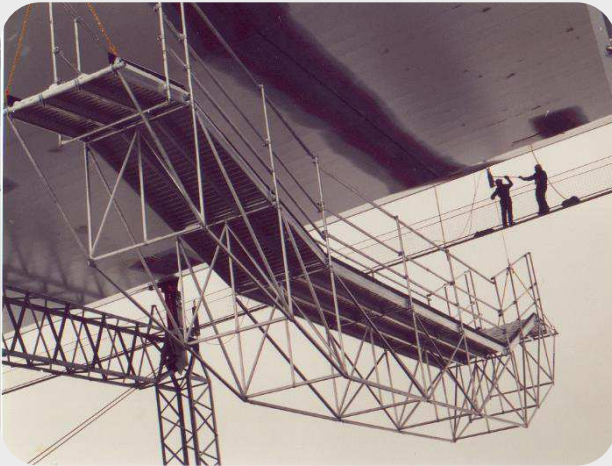
Suspended Bridge
